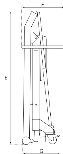
Dimensions (mm)
